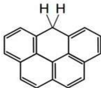
Olympicene
